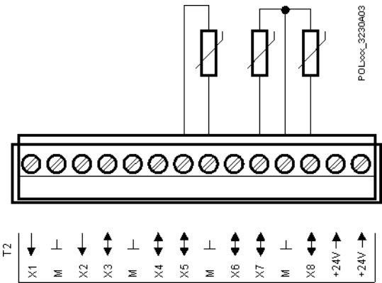
Connecting a NTC to universal I/O
