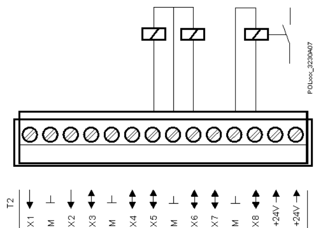
Connecting external relay to universal I/O
