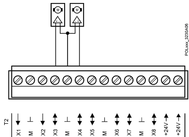
Control of actuators with 0...10V or 0...20mA analog signals
