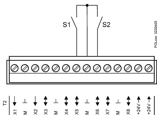
Connecting floating contacts to universal I/Os
